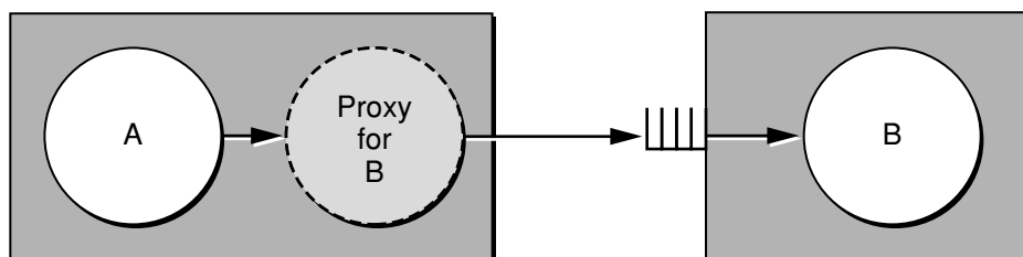
Figure 2-6 Remote Messages
