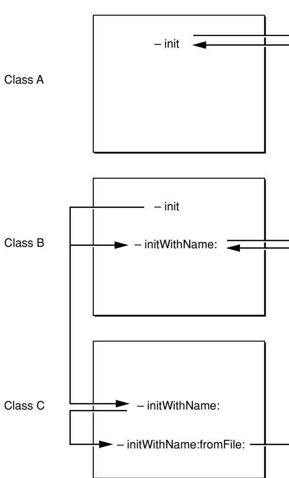
Figure 2-4 Initialization Chain
