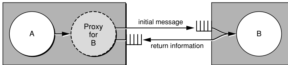
Figure 2-7 Round-Trip Message
