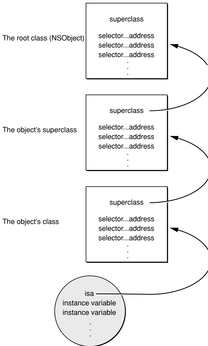
Figure 1-5 Messaging Framework
