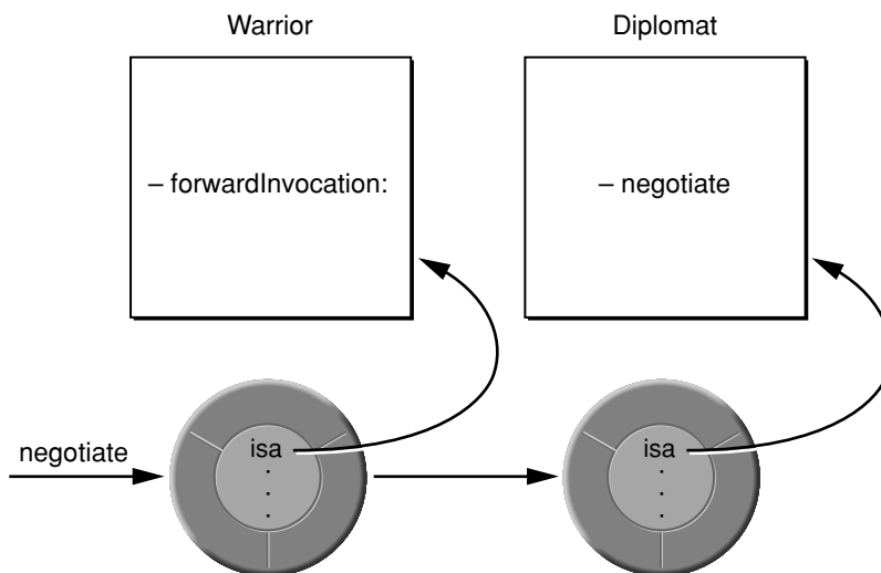
Figure 2-5 Forwarding
