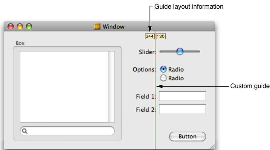
Figure 4-9 Custom layout guides
