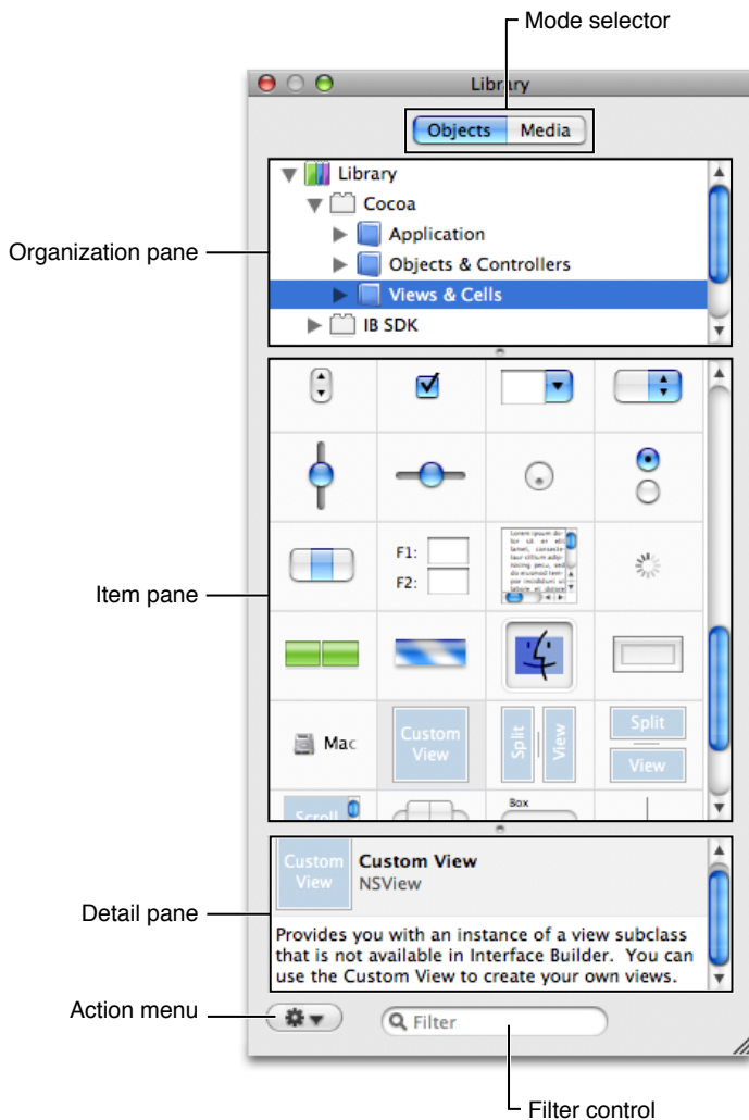
Figure 1-2 The library window
