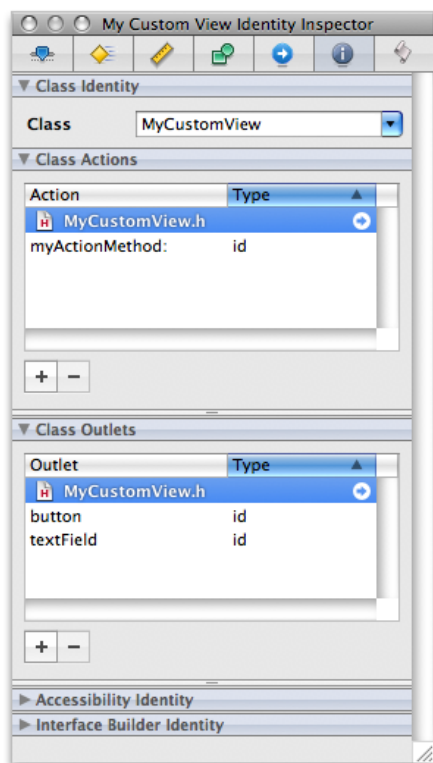
Figure 7-2 Setting the class of an object
