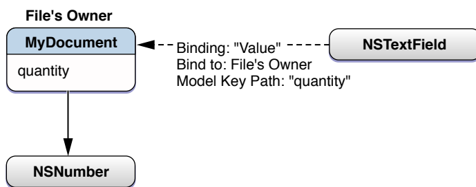
Figure 6-6 A simple bindings example
