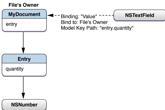
Figure 6-7 Binding through another data object
