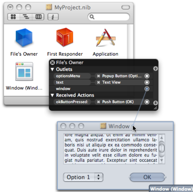
Figure 6-3 Connecting an outlet to the target
