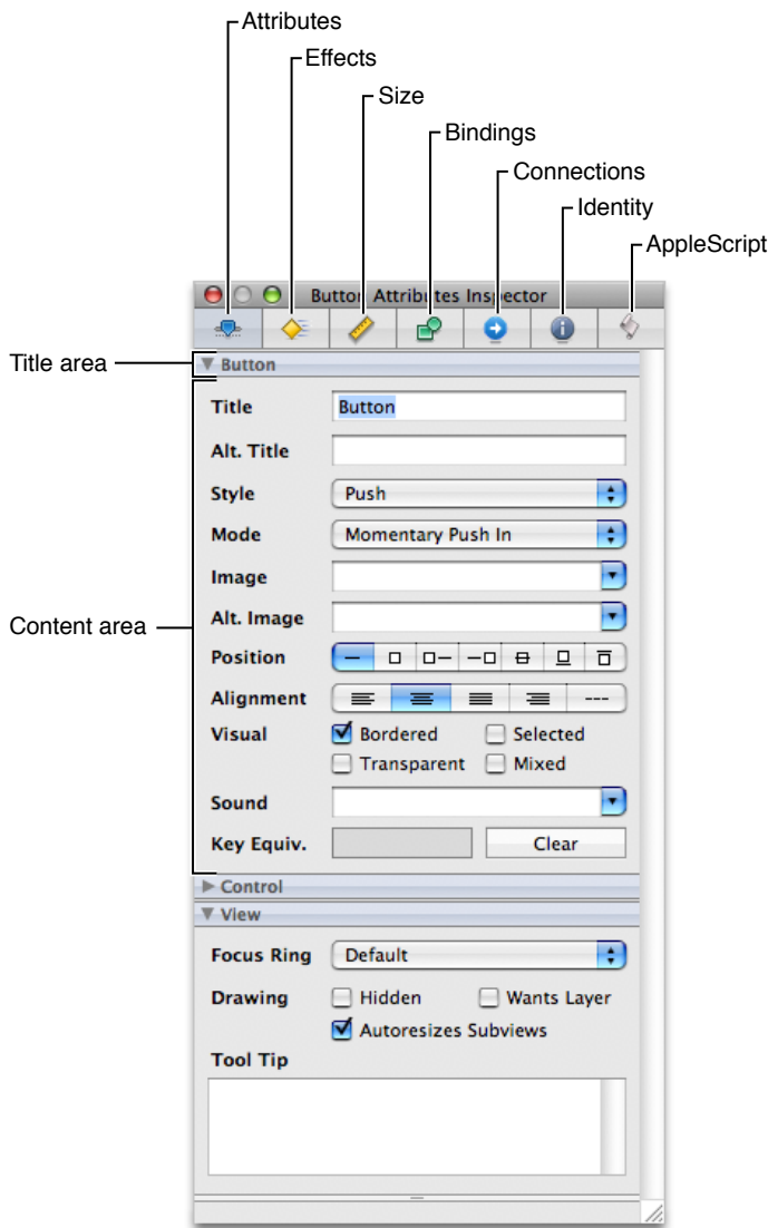
Figure 1-3 The inspector window
