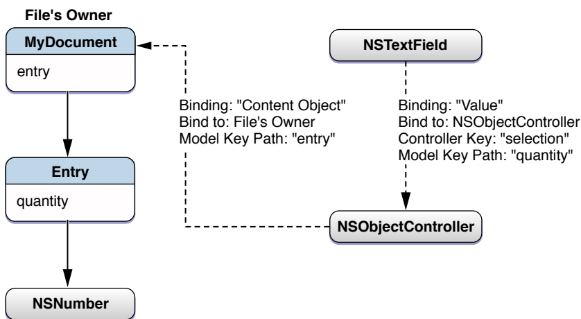
Figure 6-8 Binding through an object controller
