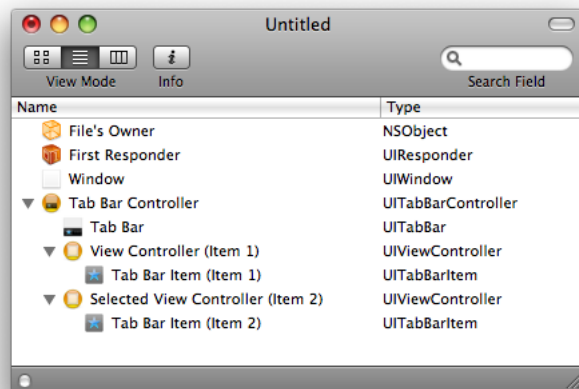
Figure 3-5 A tab bar controller and its default set of objects
