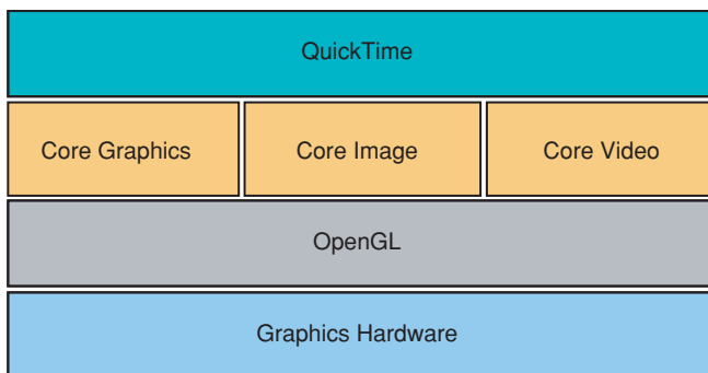
Figure 1-1 Graphics and imaging in Mac OS X
