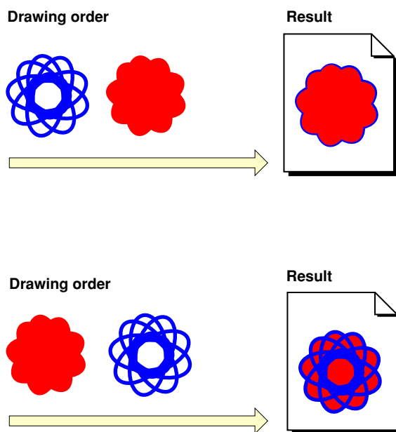
Figure 1-2 The painter’s model
