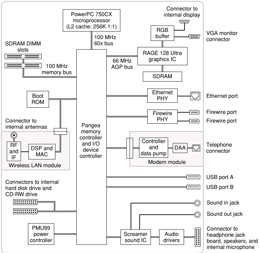
Figure 2-1 Block diagram
