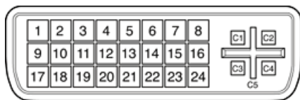
Figure 3-9 DVI-I connector
