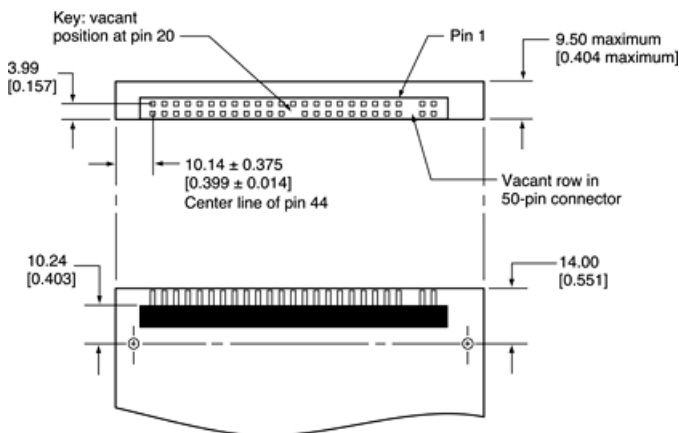
Figure 3-5 Hard disk connector and location
