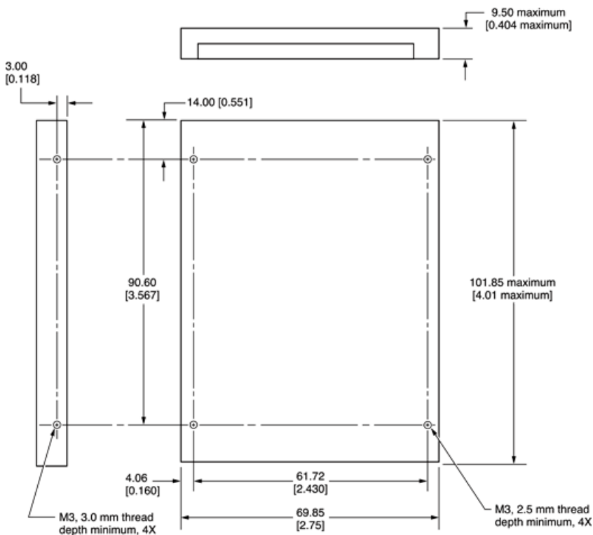
Figure 3-4 Maximum dimensions of the internal hard disk
