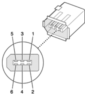
Figure 3-2 6-pin FireWire connector
