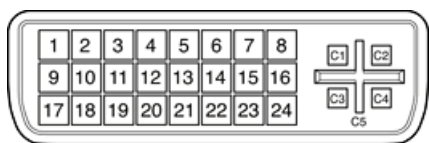
Figure 3-5 DVI connector
