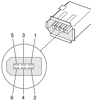
Figure 3-2 FireWire connector
