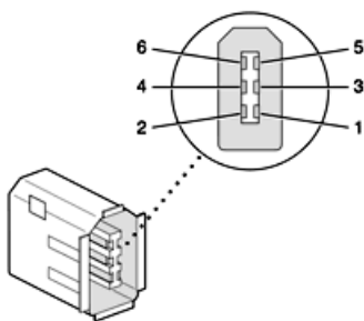
Figure 3-2 FireWire connector
