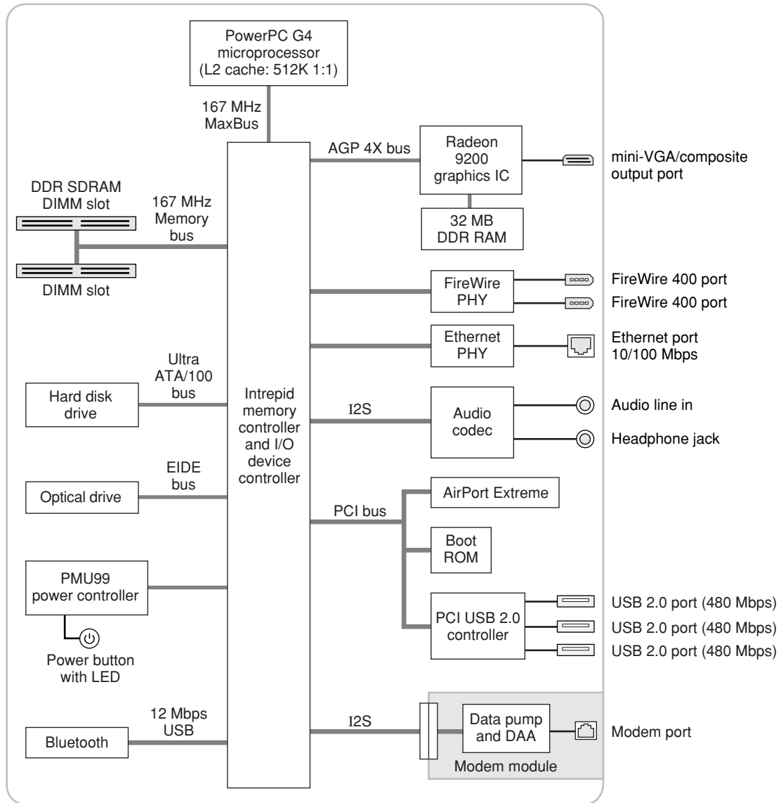
Figure 2-1 Block diagram
