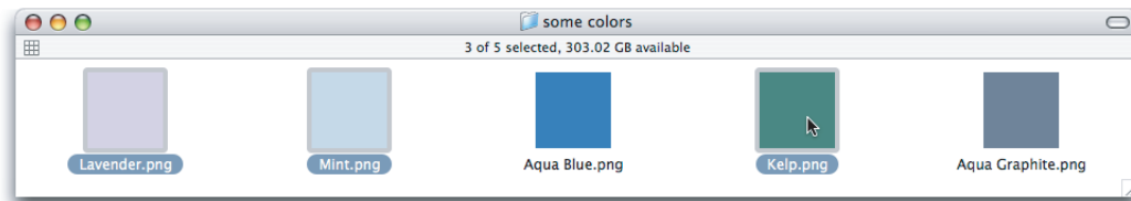
Figure 8-7 Discontinuous selection
