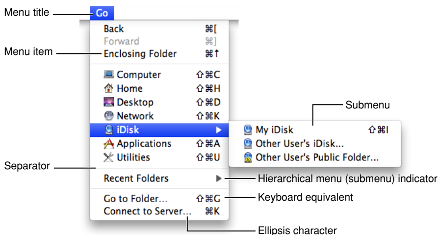
Figure 13-3 Menu elements
