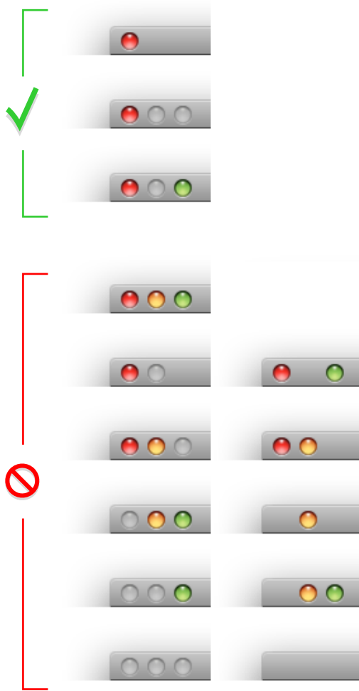
Figure 14-39 Panel controls
