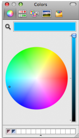
Figure 6-3 Colors window
