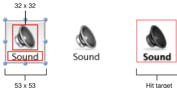
Figure 15-11 Example relationships of the icon, button, and hit-target dimensions in an icon button
