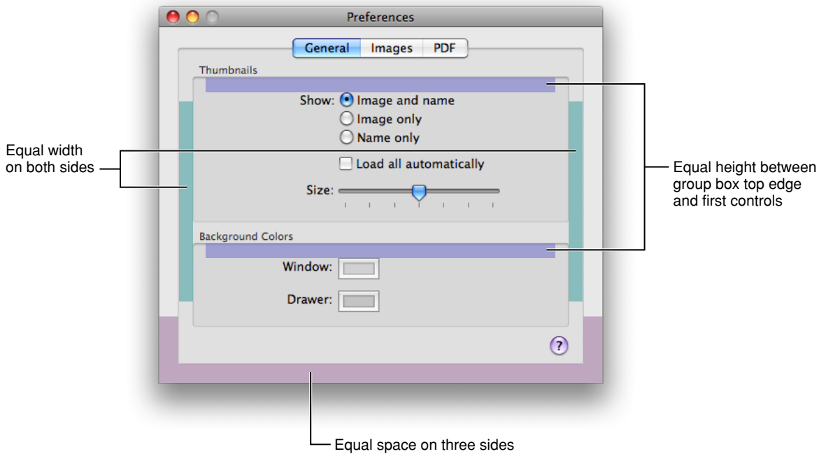
Figure 16-22 Layout dimensions using group boxes
