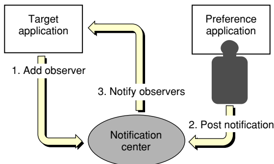
Figure 2 Distributed Notification Model
