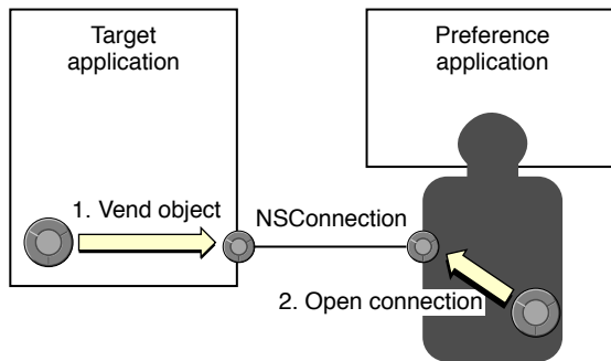
Figure 1 Distributed object architecture
