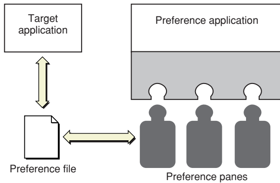
Figure 1 Plug-in architecture of preference panes
